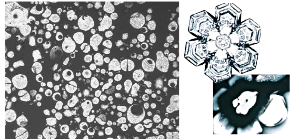
Figure 4: left: Artificial snow grains (thin section 0.03mm, 2mm x 2mm), liquid water in some grains, some grains broken from pressure during freezing process. source: Fauve et al. 2002; right: A schematic snowflake drawing compared to a micrograph of (4200x magnified) ice crystal crystallized on a Snomax nucleus (The dark speck at the flake's center). source: Scientific American Jan 07 / SNOMAX Technologies
